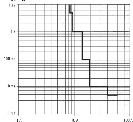
Tripping characteristic
