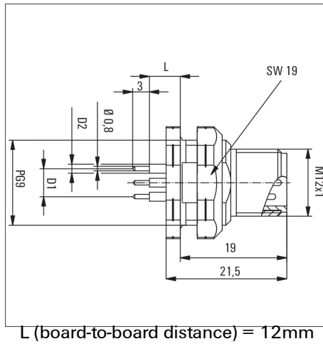
Front panel section
