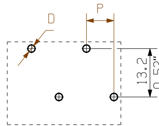
Hole pattern
