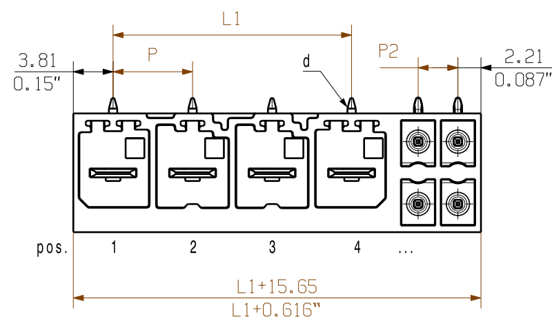
SV-SMT 7.62HP/04/270G...SC04
