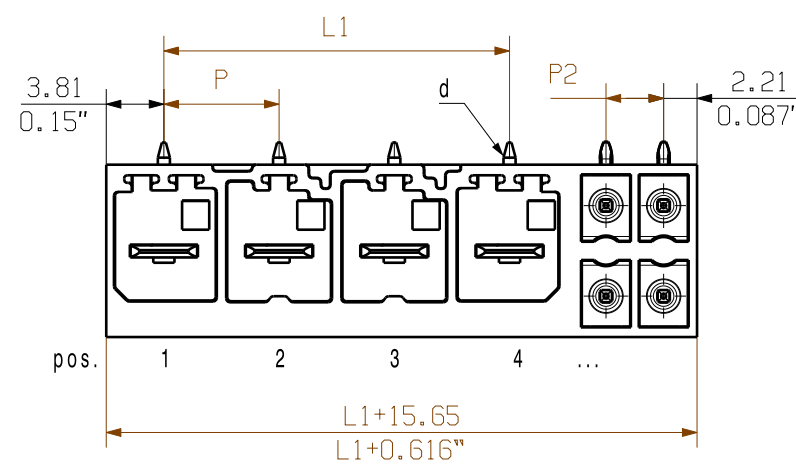
SV-SMT 7.62HP/04/270G...SC04
