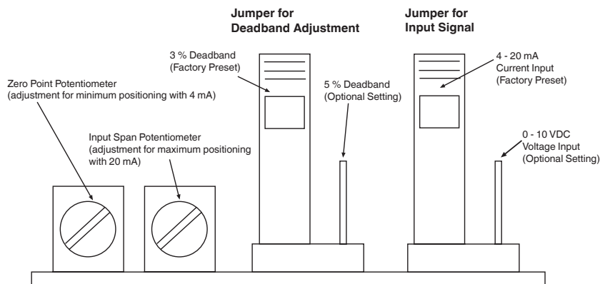
Potentiometer Adjustments and Jumpers
