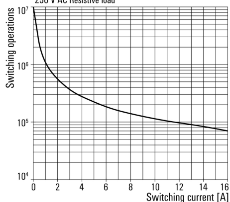
Electrical endurance
