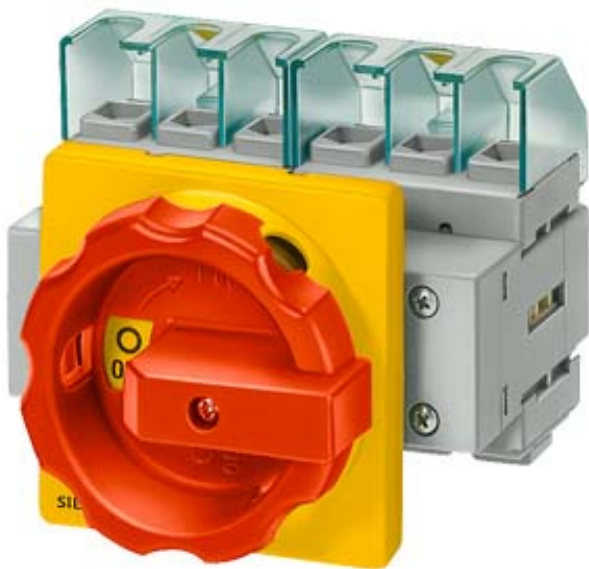
EMERG. STOP SWITCH 6-POLE IU=25, P/AC-23A AT 400V=9.5KW FRONT MOUNTING FOUR-HOLE MOUNTING ROTARY ACTUATOR RED/YELLOW (EMERG. STOP)
