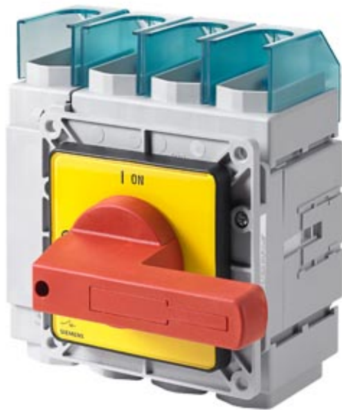
MAIN SWITCH 4-POLE FRONT MOUNTING IU=160A, P/AC-23A AT 400V=75KW ROTARY ACTUATOR RED/YELLOW (EMERG. STOP) FOUR-HOLE MOUNTING
