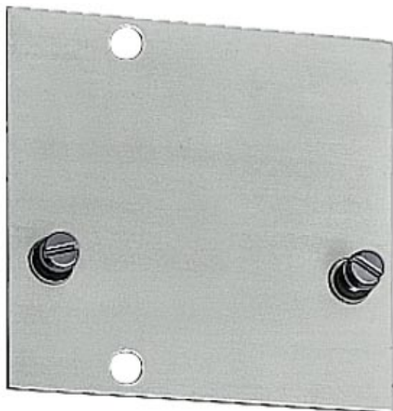
ACCESSORIES FOR FUSE SWITCH DISCONNECTORS 3NP3530 /3NP4080/3NP5060 QUICK-RETAINING PLATE CENTRE-LINE SPACING 125MM 112,5MM FOR 3NP4080/3NP5060
