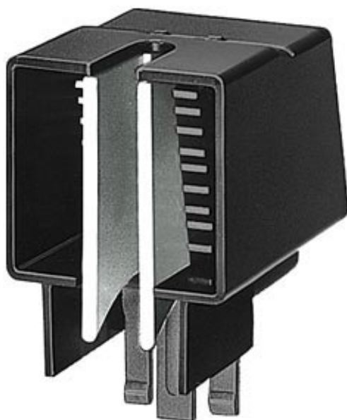
SPARE PART FOR FUSE SWITCH DISCONNECTORS 3NP52 ARC CHUTE F.RATED CURRENT 250A ARC CHUTE
