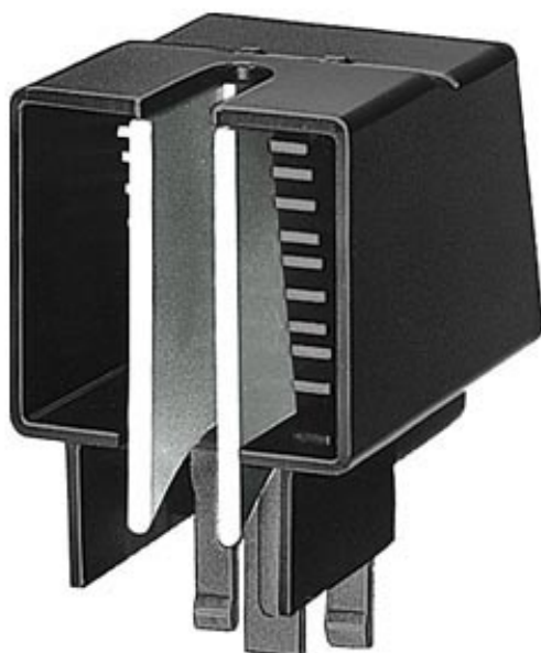
SPARE PART FOR FUSE SWITCH DISCONNECTORS 3NP53/54 ARC CHUTE ARC CHUTE
