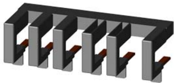
WIRING KIT, SPRING-LOADED ELECTRICAL AND MECHANICAL, INCL. MECH. INTERLOCK, FOR REVERSING STARTERS, SIZE S0
