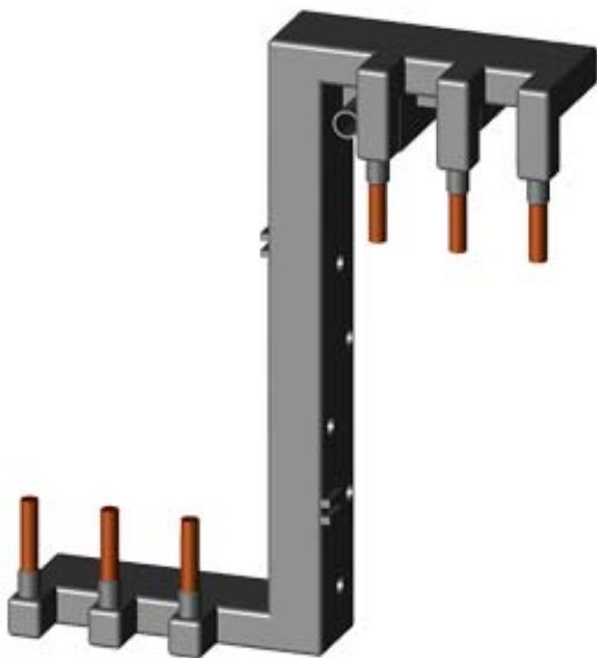
SAFETY MAIN CURRENT CONNECTOR FOR SERIES CONNECTION OF TWO 3RT202. CONTACTORS, SIZE S0 SCREW TERMINALS
