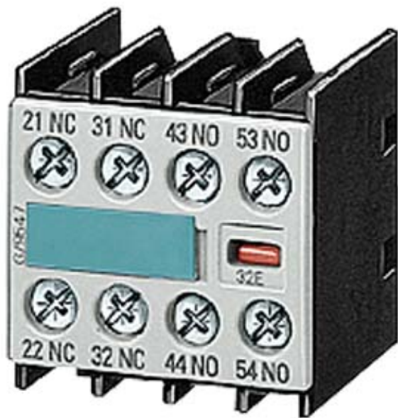
AUXILIARY SWITCH BLOCK, 22E, 1NO+2NC, DIN EN50012, SCREW CONNECTION, FOR CONTACTORS FOR SWITCHING MOTORS, 4-POLE
