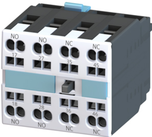
AUXILIARY SWITCH BLOCK, 22U, 2NO+2NC,, DIN EN50005, CAGE CLAMP CONNECTION, FOR SWITCHING MOTORS, SIZE S0...S12
