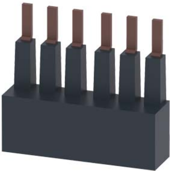
ACCESSORY FOR SIRIUS 3RM1 3-PHASE BUSBAR FOR 2 MOTOR STARTERS MODULAR SPACING 22.5MM SCREW-TYPE CONNECTION
