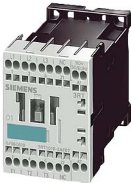
CONTACTOR, AC-3 5,5 KW/400 V, 1 NC, AC 400V 50/60HZ, 3-POLE, SIZE S00, CAGE CLAMP CONNECTION
