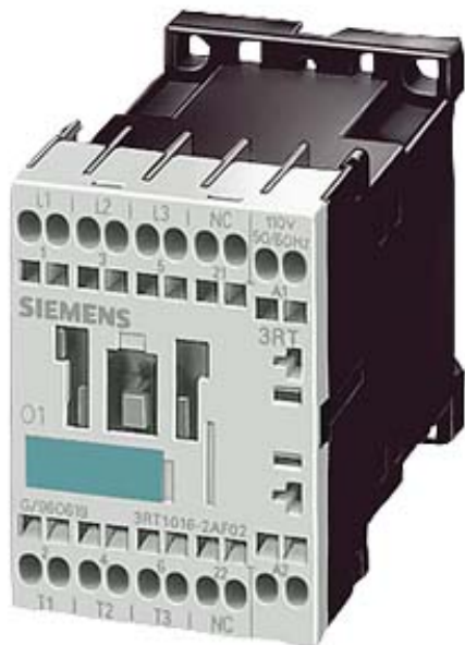
CONTACTOR, AC-3 5.5KW/400V, 1NO DC 125 V, 3-POLE, SIZE S00, CAGE CLAMP CONNECTION
