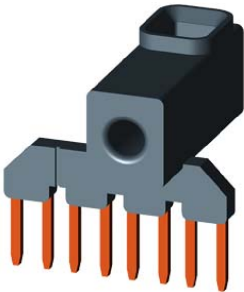
PARALLEL CONNECTION WITH TERMINAL, 4-POLE FOR 3RT101.
