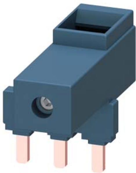
PARALLEL CONNECTION WITH TERMINAL, 3-POLE FOR 3RT103.
