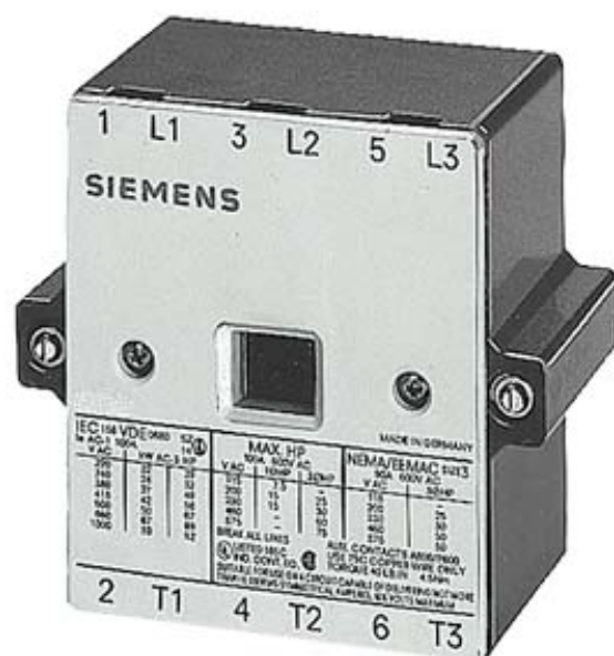
ARCING CHAMBER FOR MOD.S6 F. CONTACTOR 3RT1456, 250A/AC-1
