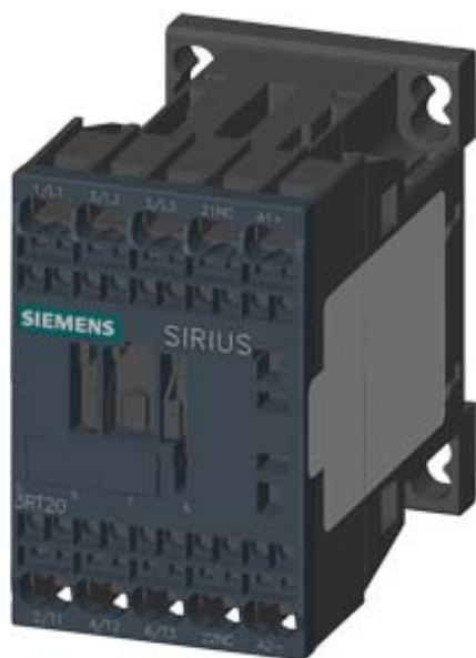
CONTACTOR, AC-3, 3KW/400V, 1NC, DC 60V, 3-POLE, SZ S00 SPRING-LOADED TERMINAL
