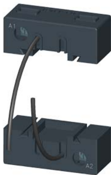
COIL CONNECTION MODULE FOR MOTOR CONTACTORS SZ S0+S2, DIAGONAL CONNECTION SCREW TERMINAL
