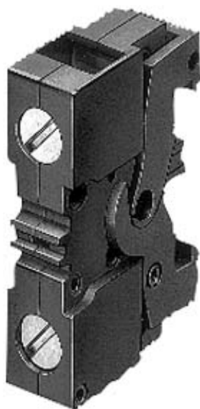
ACTUATOR-/INDICATOR COMPONENT CONTACT BLOCK WITH 1 CONTACT ELEMENT GOLD-PLATED CONTACTS SCREW TERMINAL, 1NC
