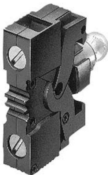
ACTUATOR-/INDICATOR COMPONENT LAMP HOLDER BA 9S WITH LAMP 24V, 3SX1344 SCREW TERMINAL CLEAR
