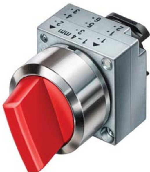
22MM METAL ROUND ACTUATOR: SELECTOR SWITCH MOMENTARY CONTACT TYPE 3 SWITCH POSITIONS I-O -II NON-ILLUMINATED WITH HOLDER BLACK
