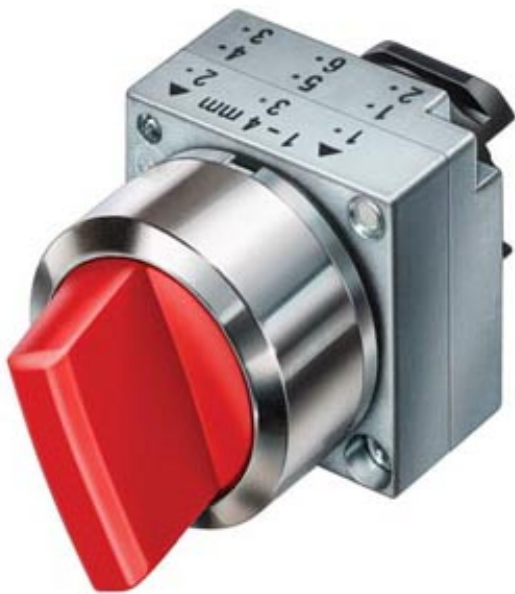
22MM METAL ROUND ACTUATOR: SELECTOR SWITCH MOMENTARY CONTACT TYPE 2 SWITCH POSITIONS O-I NON-ILLUMINATED WITH HOLDER WHITE
