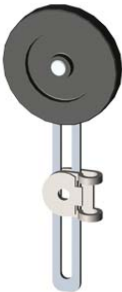
LENGTH-ADJUSTABLE TWIST LEVER FOR POSITION SWITCH 3SE51/52 METAL LEVER 100MM LONG PLASTIC ROLLER 50MM
