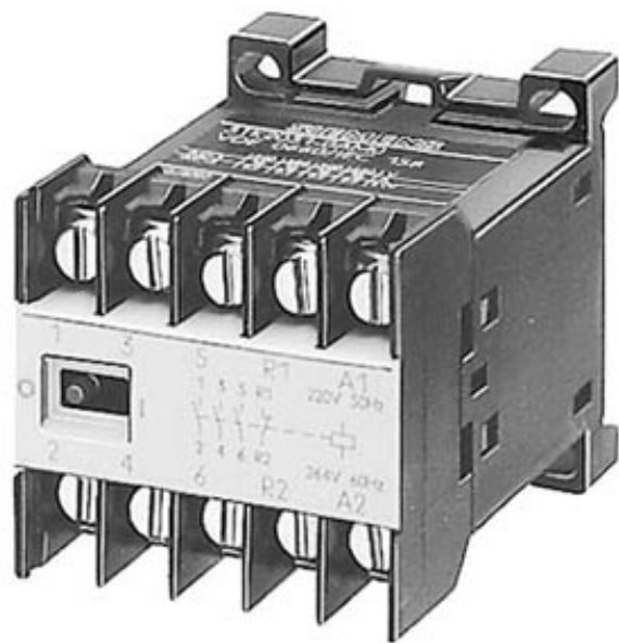
MINIATURE POWER RELAY TAB CONNECTOR, 3NO+1NC SNAP-ON MOUNTING ON STANDARD MOUNTING RAIL DC SOLENOID SYSTEM DC 24V
