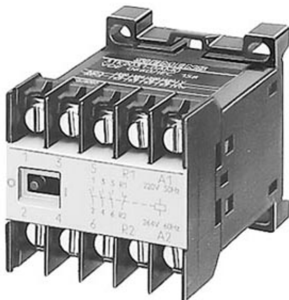
MINIATURE POWER RELAY TAB CONNECTOR, 3NO+1NC SNAP-ON MOUNTING ON STANDARD MOUNTING RAIL DC SOLENOID SYSTEM DC 110V
