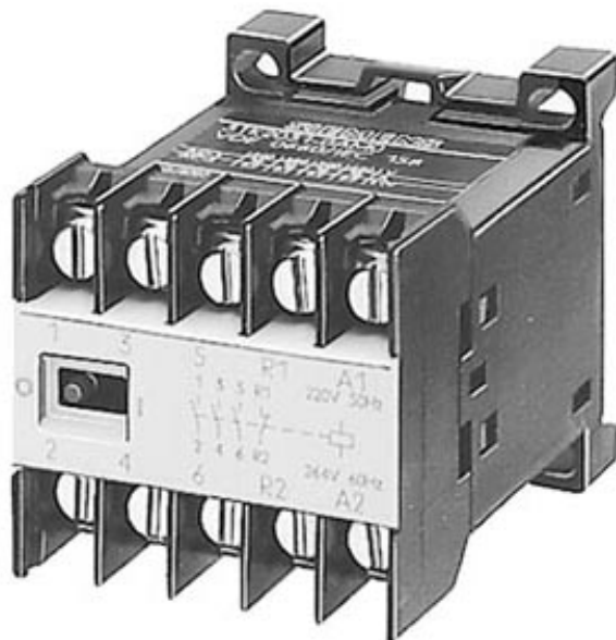
MINIATURE POWER RELAY SCREW TERMINALS, 4NO SNAP-ON MOUNTING ON STANDARD MOUNTING RAIL DC SOLENOID SYSTEM DC 24V
