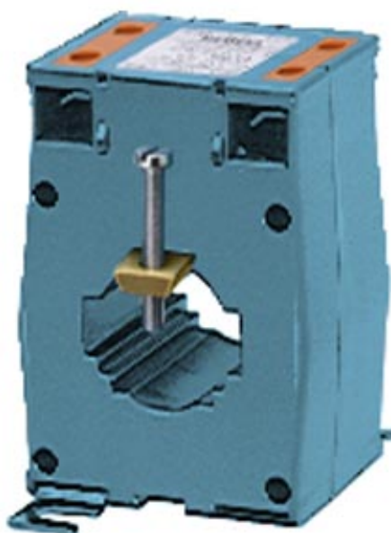
WINDOW-TYPE CURRENT TRANSFORMER, CLASS 1 250A/5A, 5VA PRIMARY CURRENT 250A, 5VA
