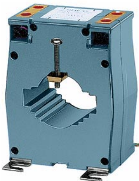
WINDOW-TYPE CURRENT TRANSFORMER, CLASS 1 500A/1A, 5VA PRIMARY CURRENT 500A, 5VA
