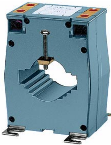
WINDOW-TYPE CURRENT TRANSFORMER, CLASS 1 750A/5A, 5VA PRIMARY CURRENT 750A, 5VA
