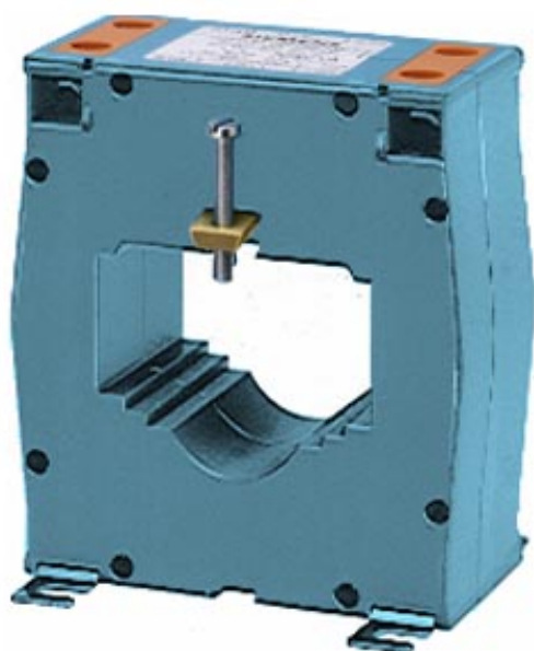
WINDOW-TYPE CURRENT TRANSFORMER, CLASS 1 1250A/1A, 10VA PRIMARY CURRENT 1250A, 10VA
