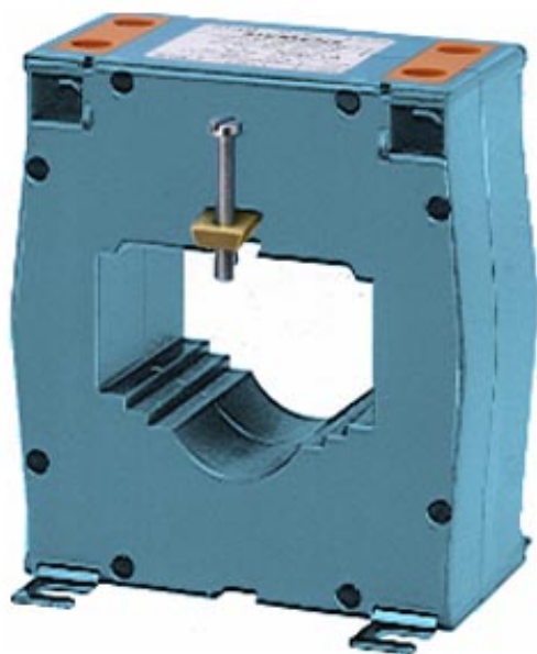
WINDOW-TYPE CURRENT TRANSFORMER, CLASS 1 1500A/5A, 10VA PRIMARY CURRENT 1500A, 10VA
