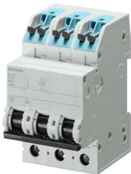
CIRCUIT BREAKER 400V 6KA, 3-POLE, C, 10A, D=70MM WITH SCREWLESS TAP-OFF TERMINAL
