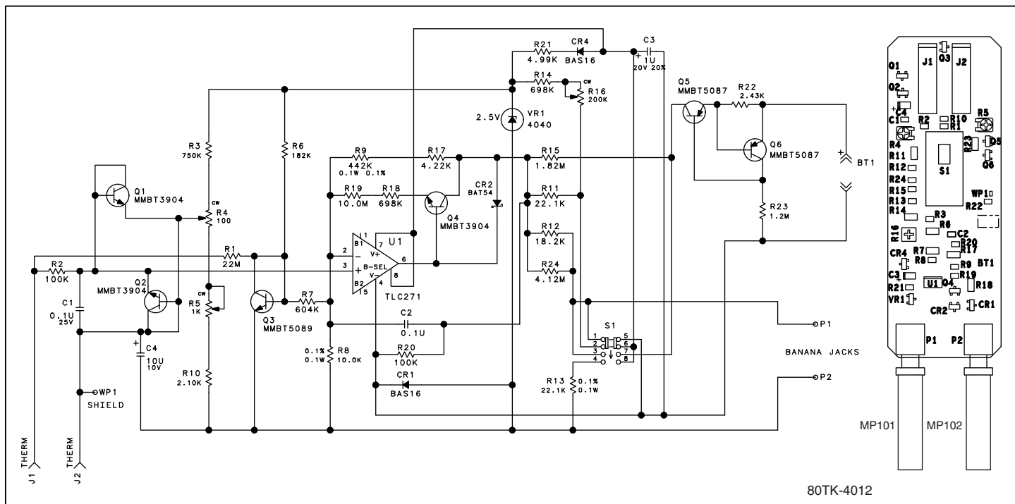
80TK Schematic Diagram
