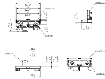
DIRECT MOUNTING
