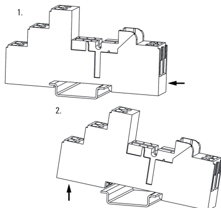
Unlatching socket
