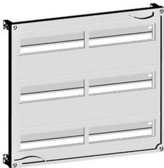
ALPHA 160 DIN, ASSEMBLY KIT F. MODULAR INSTALLATION DEVICES, TIER SPACING 150MM, H=450 W=250
