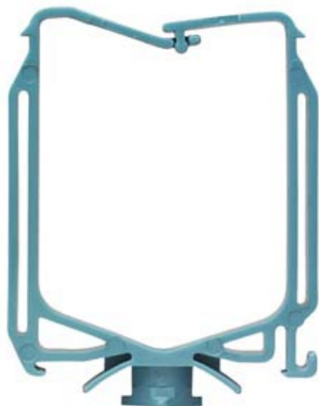
ALPHA 400/630 CABLE HOLDER ON STANDARD MOUNTING RAIL MIN. ORDER QUANTITY 200 UNITS
