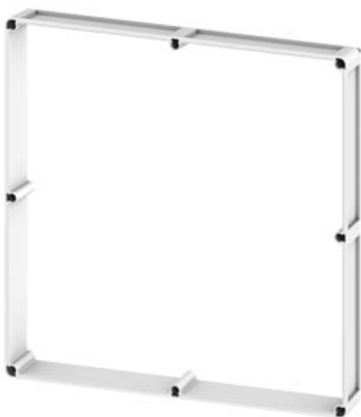
INTERMED. FRAME F. INCREASING MOUNTING DEPTH BY 92.5 MM FOR ENCLOSURE SIZE 4
