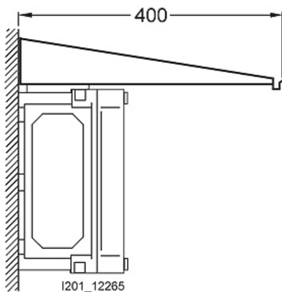
DISTRIBUTION SYSTEM 8HP RAIN CANOPY FOR WALL-MOUNTING F. 1 ENCLOSURE WIDTH
