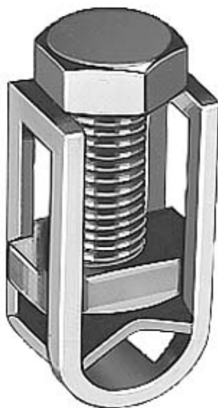
TERMINAL 1-POLE, FOR BUSBAR 12 X 5 CONDUCTOR CONNECTION 1 X 16- 70MM 2
