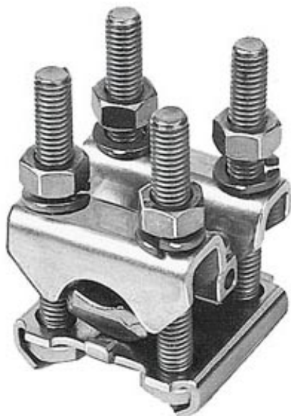
TERMINAL 1-POLE, FOR BUSBAR 20 X 8 CONDUCTOR CONNECTION 1 X 50- 185MM2
