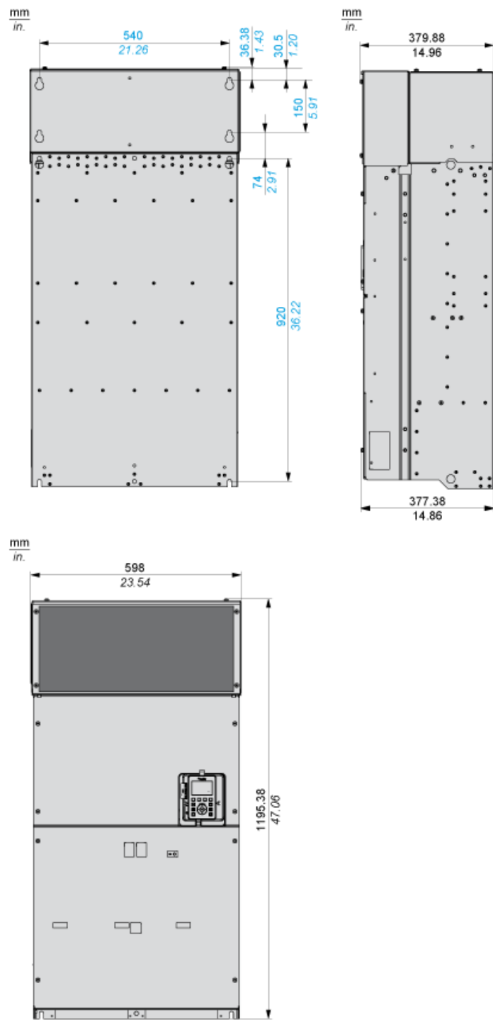
Rear, Right and Front Views
