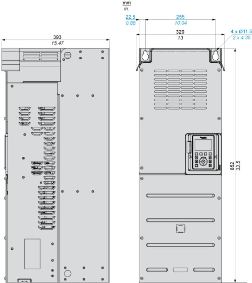
Right and Front View
