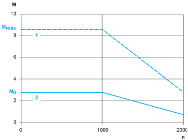
Servo Motor with LXM23•U04M3X Servo Drive
